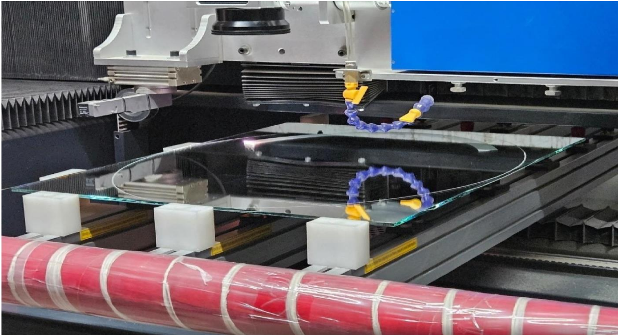
OUR CNC LASER FROSTING A GLASS PANEL · PANCHKULA WORKSHOP
